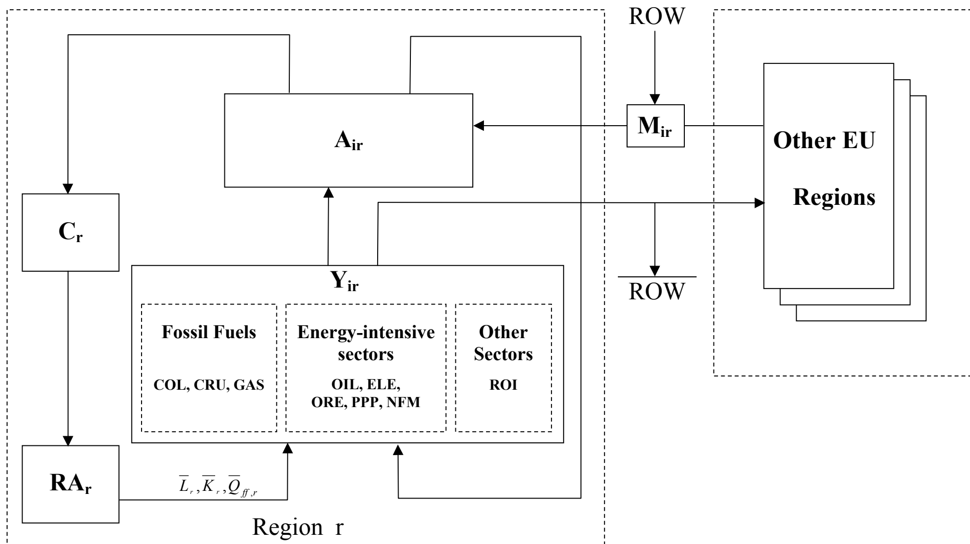
Figure 2: Diagrammatic CGE model structure
